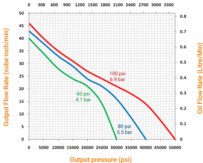
OIL FLOW RATE - STANDARD
