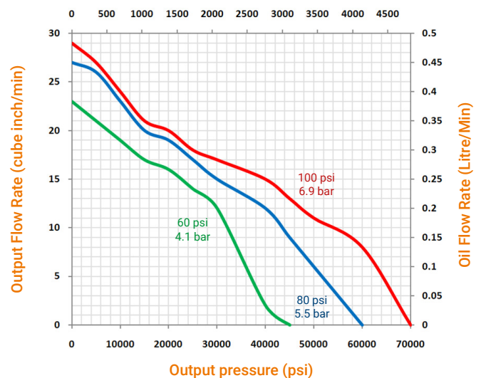
OIL FLOW RATE - HIGH FLOW
